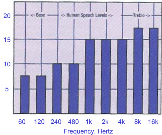
Typical Silencing Curve Tube Silenced Air Intake Filters (Each 10dB reduction lowers perceived "loudness" by half)
