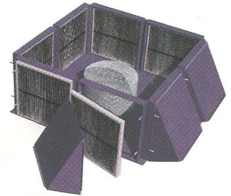
Note 304SS safety cage downstream of panel filters. Helps prevent leaves, pens, hats, and other debris from traveling into the compressor, blower, or turbine intake at filter change out!!!
