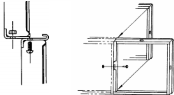
NS-100 FILTER HOLDING FRAME
