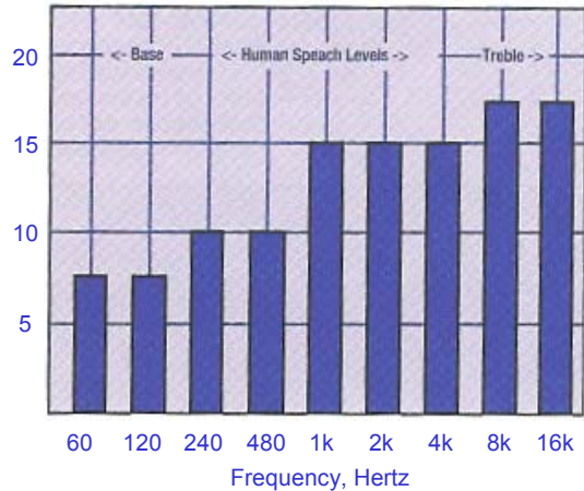
Typical Silencing Curve Tube Silenced Air Intake Filters (Each 10dB reduction lowers perceived "loudness" by half)
